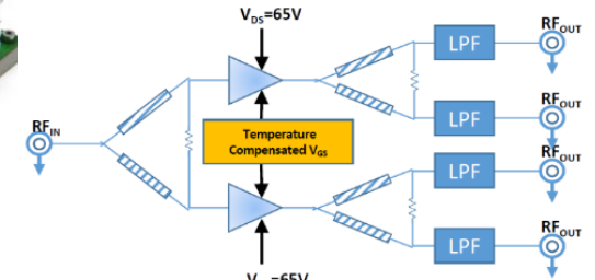
BLOCK DIAGRAM
