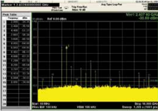
IF output reflection spectrum with conventional filter
