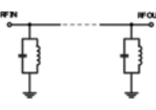
Simplified Schematic
