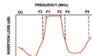
Typical Frequency Response
