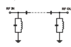
Simplified Schematic
