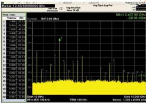
IF output reflection spectrum without filter
