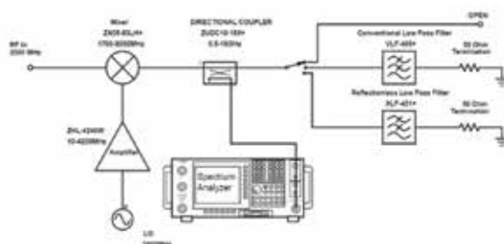
Application circuit test setup
