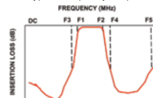
Typical Frequency Response
