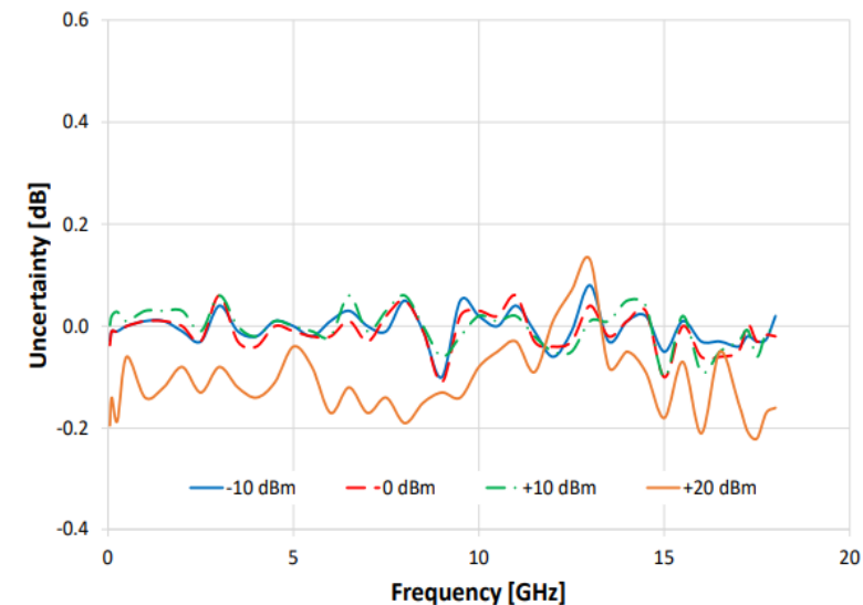
Uncertainty in Power Measurement @ High Power Input
