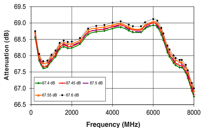
Attenuation relative to I.Loss Fine resolution around Atten. 67.5 dB
