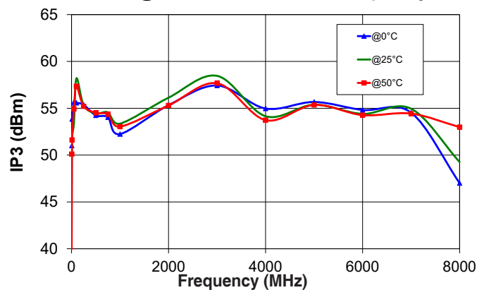
IP3 @ 0dB Attenuation vs. Frequency
