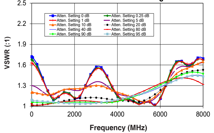
Output VSWR vs. Frequency over Attenuation settings
