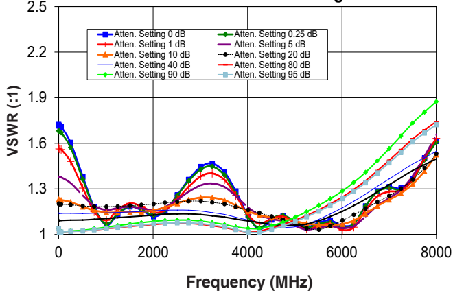
Input VSWR vs. Frequency over Attenuation settings
