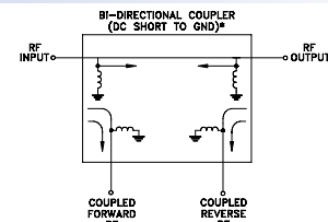
ELECTRICAL SCHEMATIC SYDC SERIES
