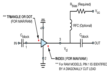
RAM, MAR, MAV, VAM TYPICAL BIASING CONFIGURATION
