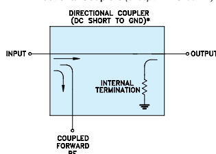
Directional Couplers (except P4DC-30A-2)
