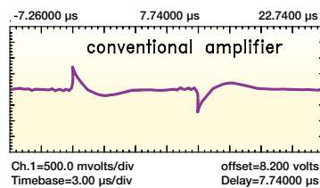
TYPICAL AMPLIFIER RESPONSE TO PULSE INPUT
