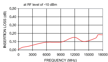
TYPE-N/SMA INSERTION LOSS
