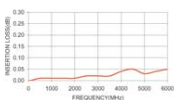
TYPE-N/TYPE-N INSERTION LOSS
