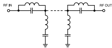
FUNCTIONAL SCHEMATIC
