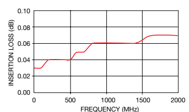
TYPE-N/BNC INSERTION LOSS
