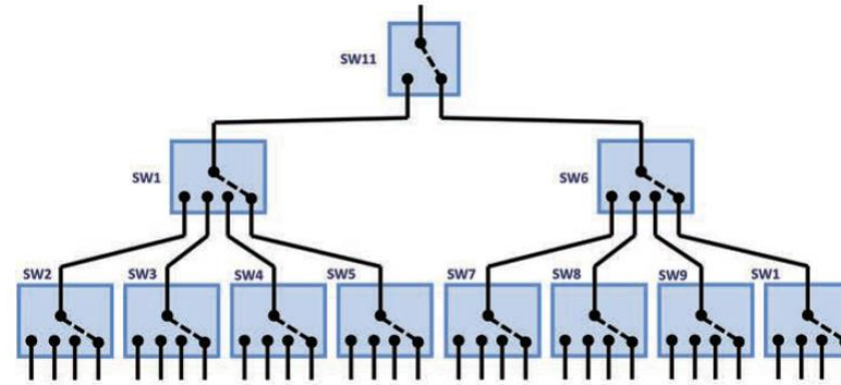
Single Pole 32 Throw (SP32T) Switch
