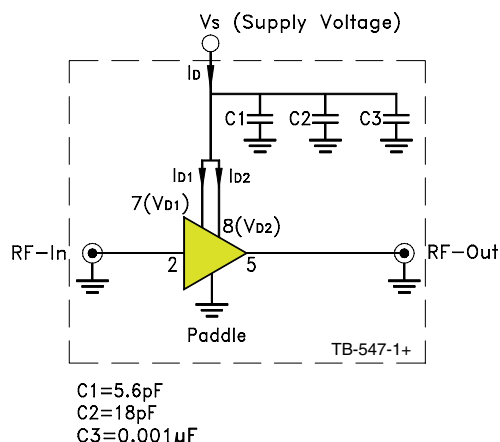
Fig 1. Block Diagram of Test Circuit used for characterization. (DUT soldered on Mini-Circuits Characterization Test Board TB-547-1+) Gain, Output power at 1dB compression (P1dB), Noise Figure, Output IP3 (OIP3) are measured using Agilent's N5242A PNA-X microwave network analyzer.
